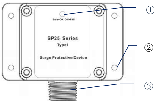
Fig 1: Diagram of SP25 Series
