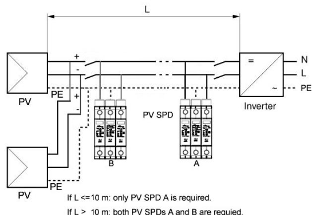
Fig 3: Positions of SPDs (Y configuration) in the DC part stipulated in Guide IEC 61643-32
