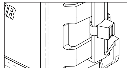
Figure 5 - Tie wrap placement
