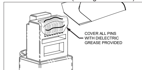
Figure 8 - Grease application
