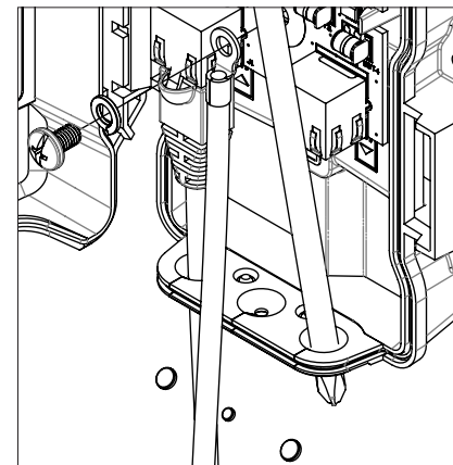
Figure 4 - Cable installation
