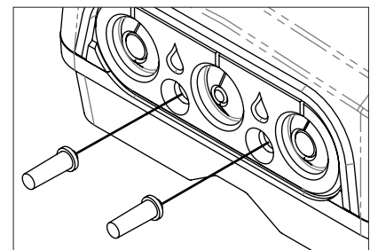
Figure 6 - Drain plug removal
