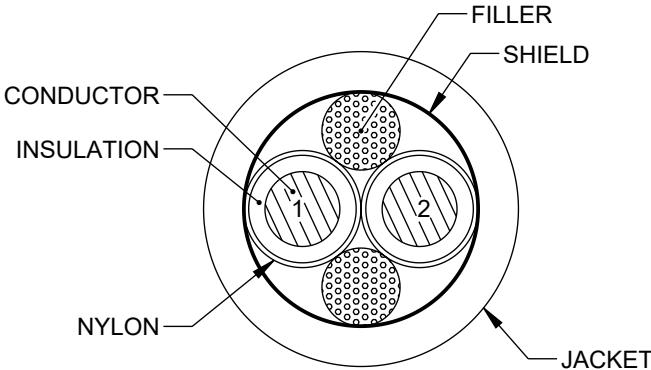
CROSS-SECTIONAL VIEW
