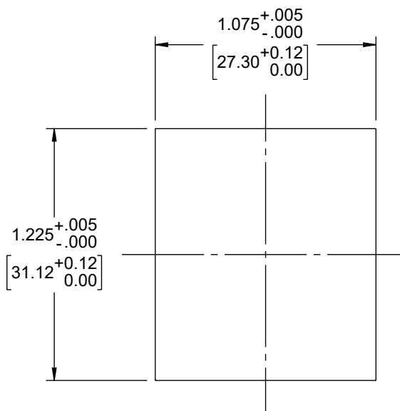
PANEL DETAIL
